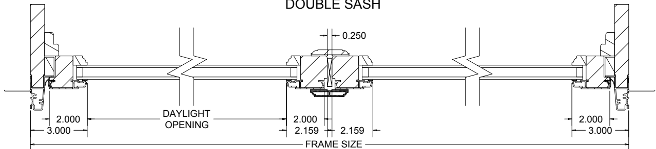
NARROW STILE TRANSOM - DOUBLE SASH
