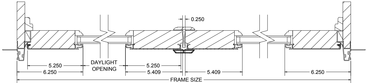
WIDE STILE TRANSOM - DOUBLE SASH
