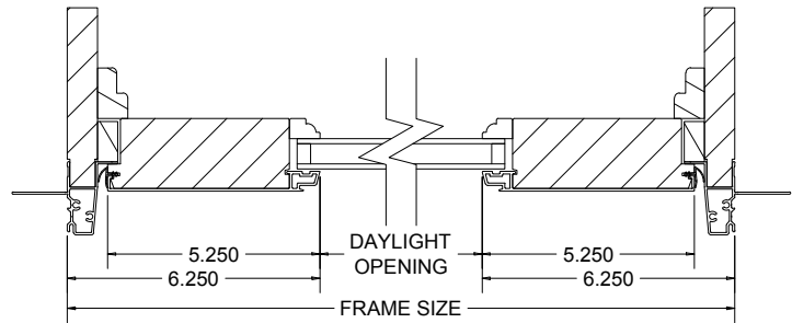
WIDE STILE TRANSOM - SINGLE SASH
