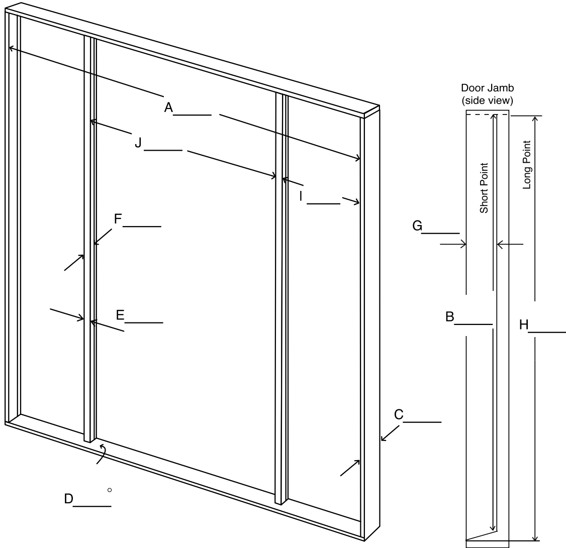
Single door with two sidelites continuous head & sill.
