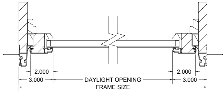
NARROW STILE TRANSOM - SINGLE SASH
