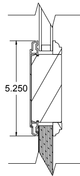
MID-RAIL WITH ALUMINUM CLAD PANEL
