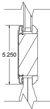
MID-RAIL WITH WOOD RAISED PANEL
