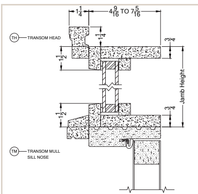
Rectangle w/Sill Nose
