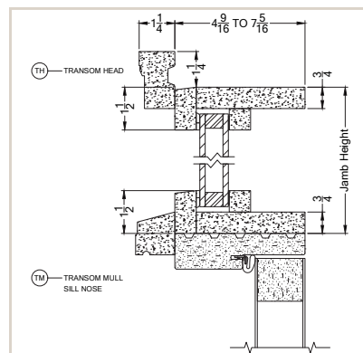
Curved Transom Design
