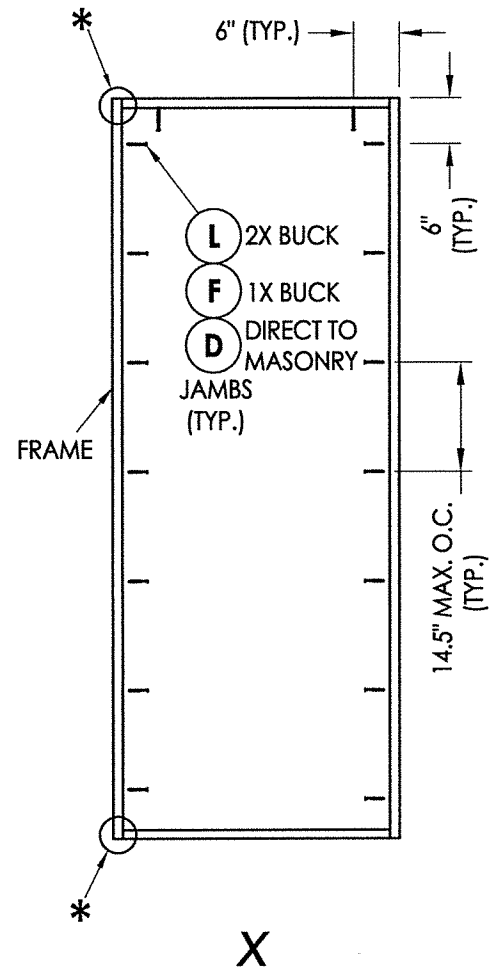
FRAME ANCHORING
