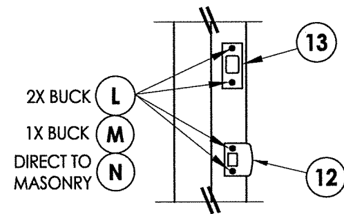
LATCH & DEADBOLT DETAIL
